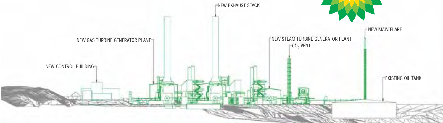
DF1 cross section looking north.
